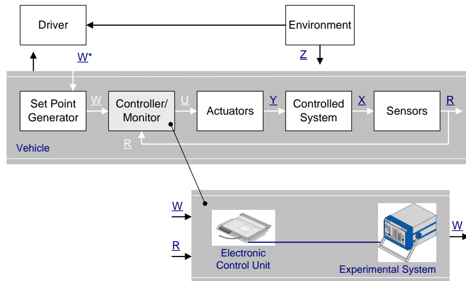
Fig. 3-2 A typical rapid prototyping system
