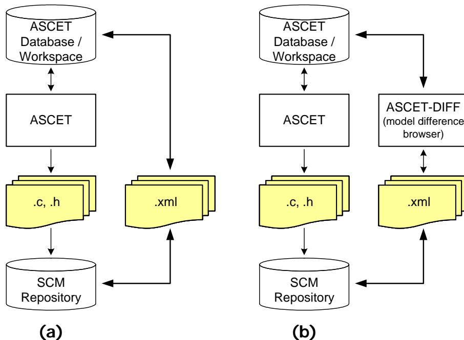
Fig. 3-5 ASCET-SCM interface with (b) and without (a) ASCET-DIFF
