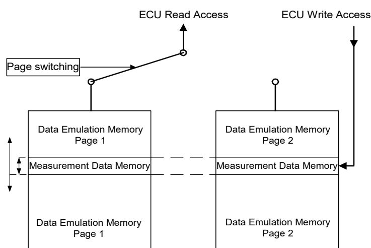
Fig. 4-3 Data Emulation and Measurement Data Memory: 2 Pages with 512 kByte each
