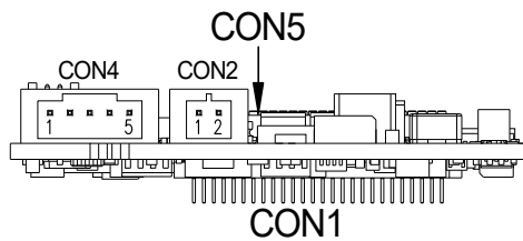
Fig. 4-6 Power Supply Connector CON2
