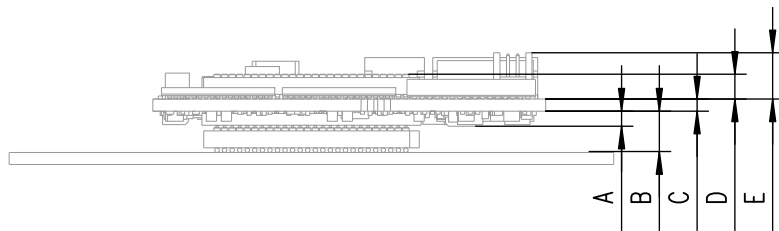
Fig. 7-4 Microcontroller with Socket Adapter mounted (ETK-T1.1A and ETK-T1.1B)
