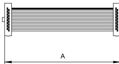
Fig. 8-13 ETAF5 Flatcable
