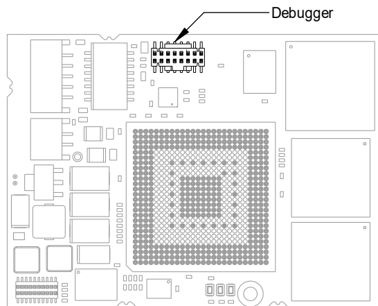
Fig. 4-8 Location of the Debugger Interface
