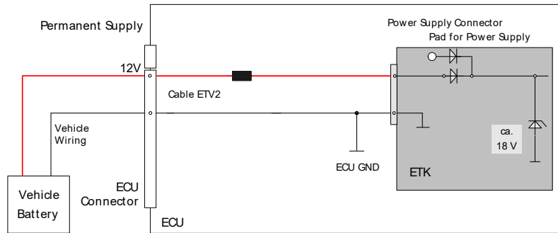
Fig. 5-4 Permanent Power Supply inside ECU available
