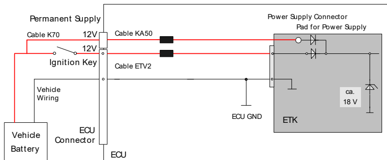
Fig. 5-5 Permanent Power Supply inside ECU not available
