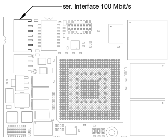
Fig. 4-7 Location of the Serial ETK Interface
