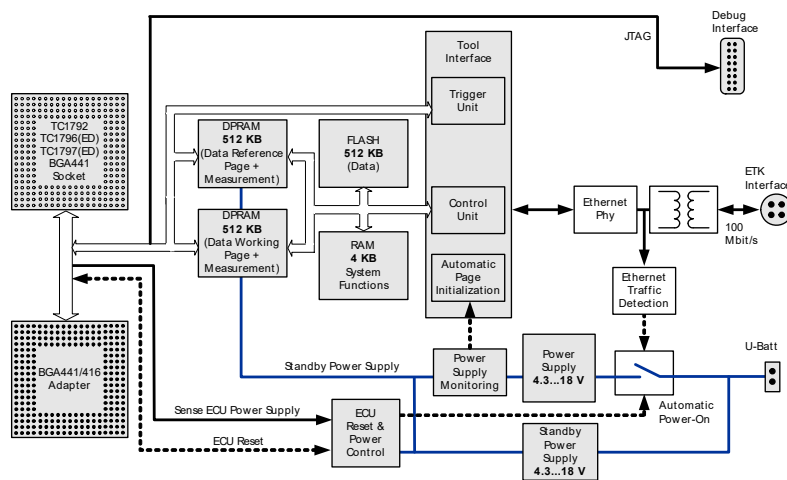
Fig. 4-1 ETK-T1.1 Architecture
