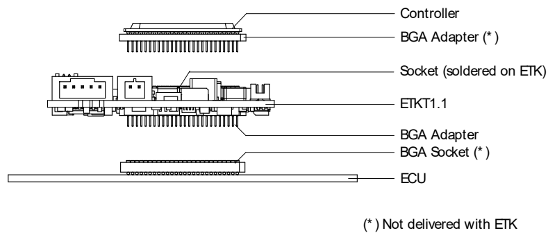
Fig. 5-1 ETK-T1.1 Connection to the ECU
