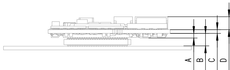
Fig. 7-6 Microcontroller directly soldered (ETK-T1.1C and ETK-T1.1D)
