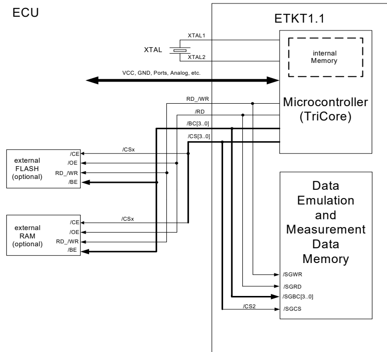
Fig. 4-2 System with internal and external Memory
