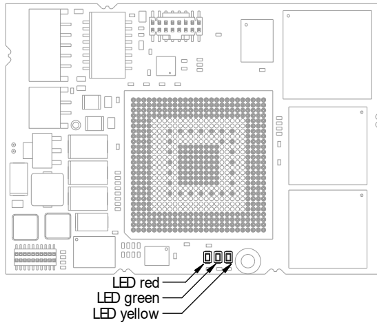
Fig. 4-9 Status LEDs
