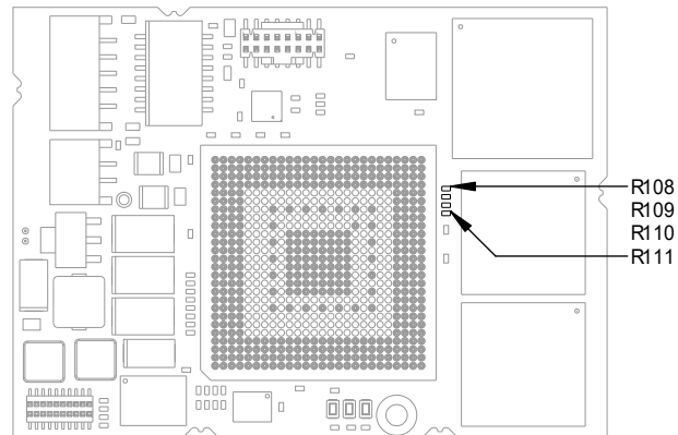
Fig. 4-10 Chip Select Configuration Bridge
