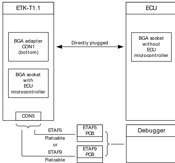
Fig. 5-3 ETK-T1.1 Connection to the ECU and to the Debugger
