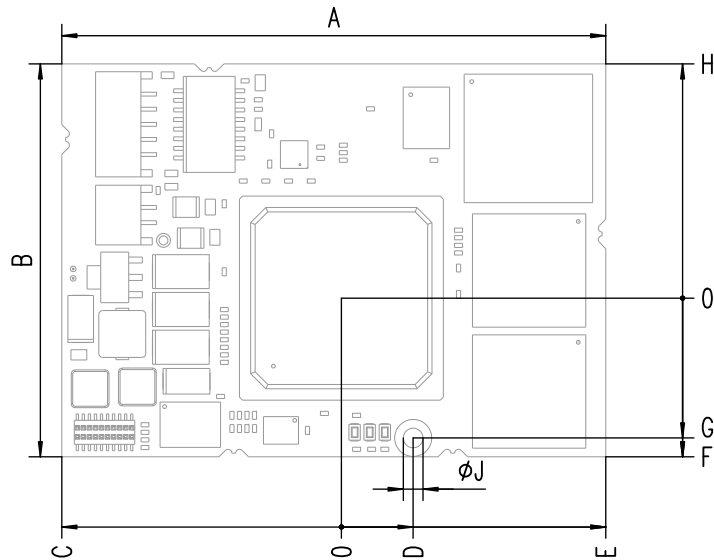
Fig. 7-5 ETK-T1.1C and ETK-T1.1D Dimensions - Top View
