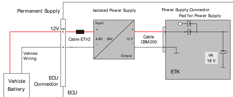
Fig. 5-6 Isolated Power Supply inside ECU
