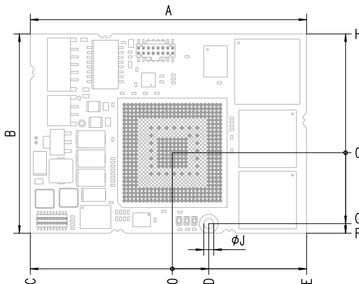
Fig. 7-3 ETK-T1.1A and ETK-T1.1B Dimensions - Top View
