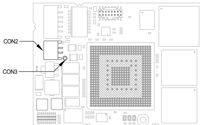
Fig. 4-5 Power Supply Connectors CON2 and CON3
