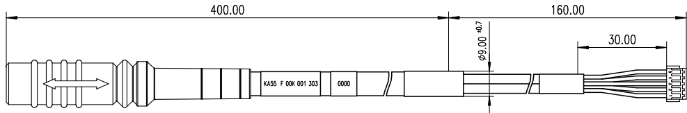
Figure 3: Mechanical Dimensions
