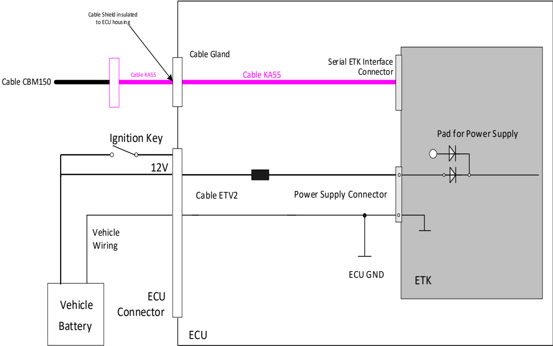
Figure 2: Installation
