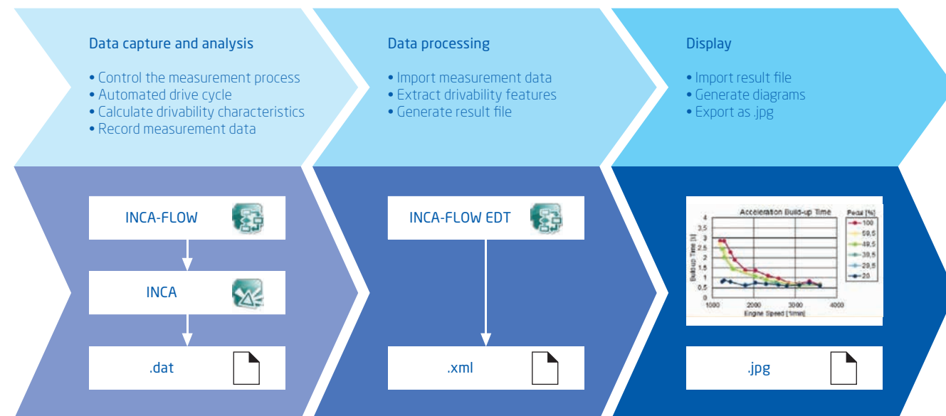
EDToolchain – from the performance of driving maneuvers to the capture and analysis of measurement data and the presentation of results
