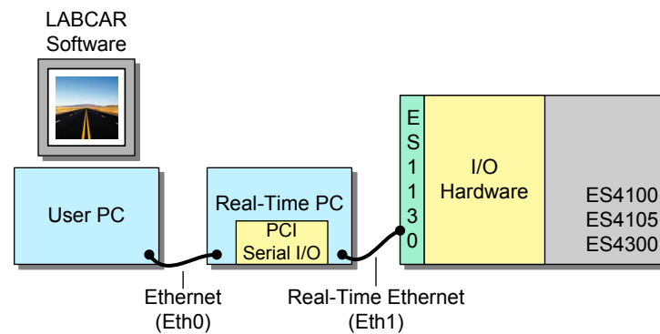
Fig. 1-1 RTPC System
