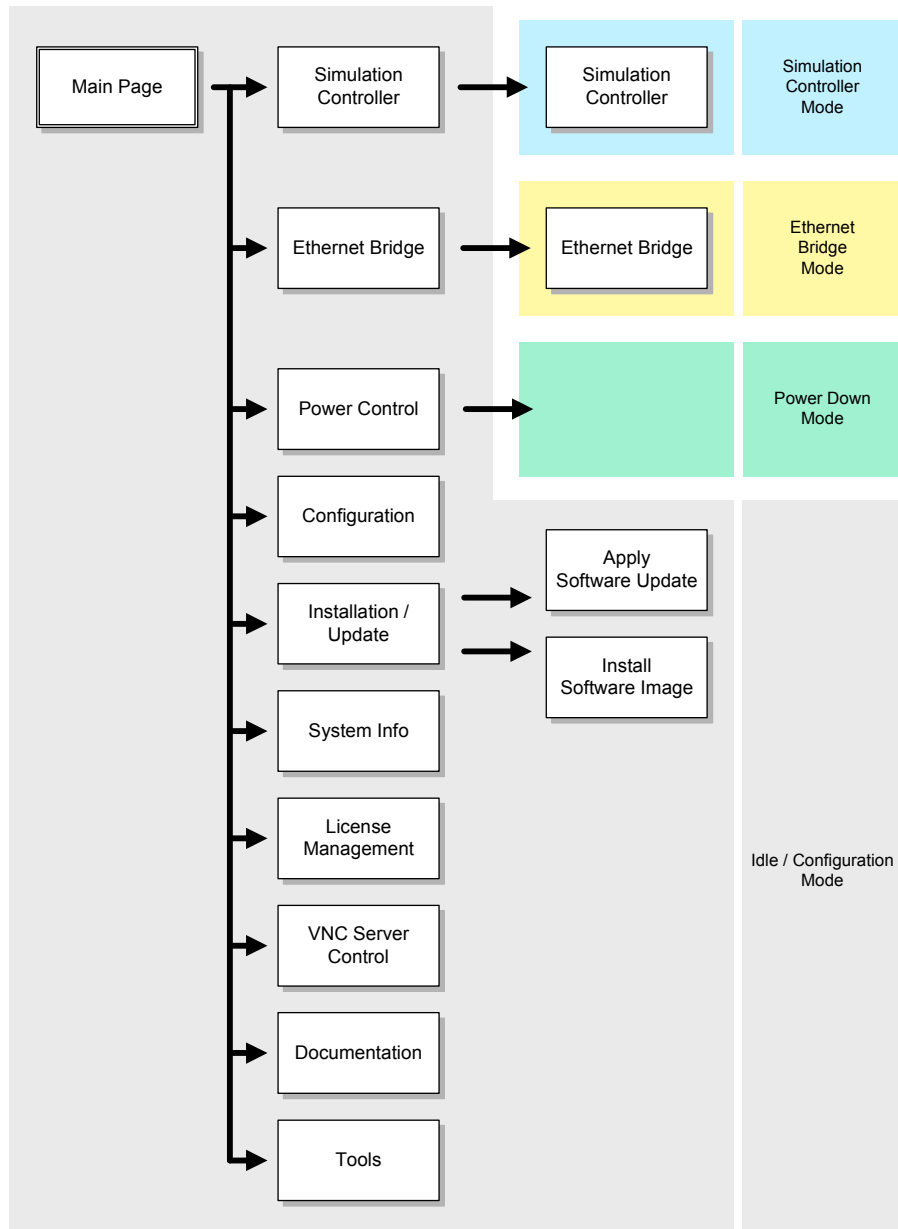
Fig. 4-2 Structure of the Web Interface
