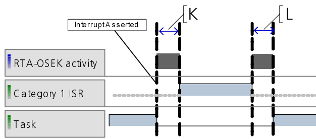
Figure 1 - Category 1 interrupt with return to interrupted task
