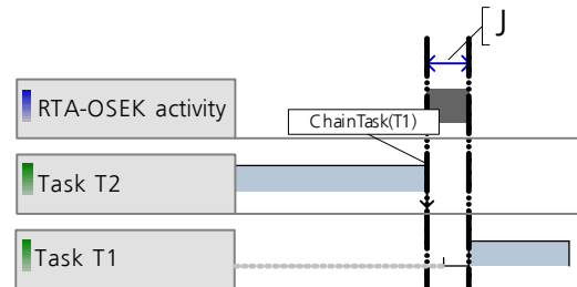
Figure 6 - Task chaining
