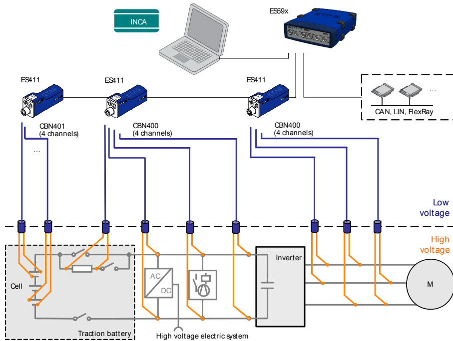
Fig. 2-3 Use of the CBN401.1 and the CBN401.1 in the high-voltage on-board system
